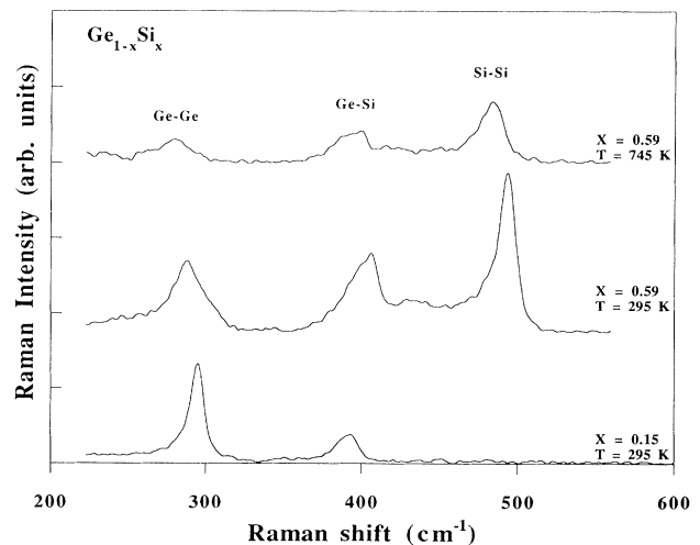
FIG. 1. Typical Raman spectra of \text{Ge}_{1-x}\text{Si}_x alloys, with the three modes denoted.
