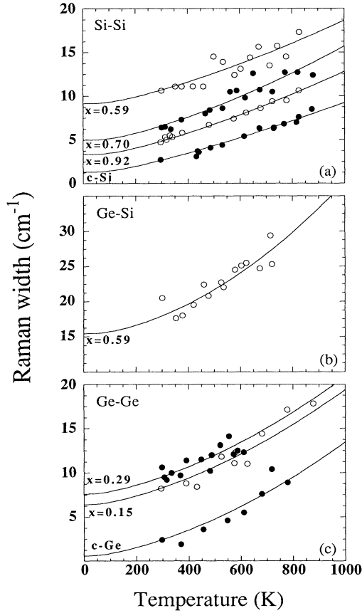
FIG. 4. Raman linewidths of the three \text{Ge}_{1-x}\text{Si}_x alloy modes as a function of temperature, for different alloy concentrations. The experimental uncertainty in the width is \sim \pm 4\% . The solid lines are fit using Eq. (5), with parameters given in Table III for each mode and composition, with the exception of curve drawn through the x=0.29 Ge-Ge data. For ease of viewing, this curve was plotted with the B_{1i} and B_{2i} of the x=0.15 Ge-Ge mode. The data for c -Ge were corrected by using the 2.3\text{-cm}^{-1} instrumental linewidth for that run, and not the average value ( 2.8\text{ cm}^{-1} ) used for the other runs.
