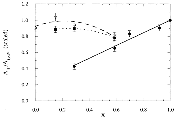
FIG. 5. Scaled values of A_{ii} for the three modes, normalized to the value in c -Si. The scaling relationship for the quartic anharmonic parameters, M_i^2 \omega_{0i}^2 A_{ii} , is used. The solid circles, solid squares, and open circles represent the Si-Si, Ge-Si, and the Ge-Ge modes, respectively. The curves through the points, which are solid, dotted, and dashed, respectively, are meant to aid viewing.
