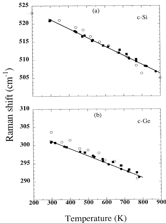
FIG. 2. Raman shifts of (a) c -Si and (b) c -Ge as a function of temperature from several experiments. The squares are data from Ref. 3, the open circles in (a) and (b) are data from Refs. 4 and 7, respectively, and the solid circles are from this experiment, for which the uncertainty is \pm 0.25 \text{ cm}^{-1} for T < 600 \text{ K} , and \pm 0.50 \text{ cm}^{-1} for T > 600 \text{ K} .
