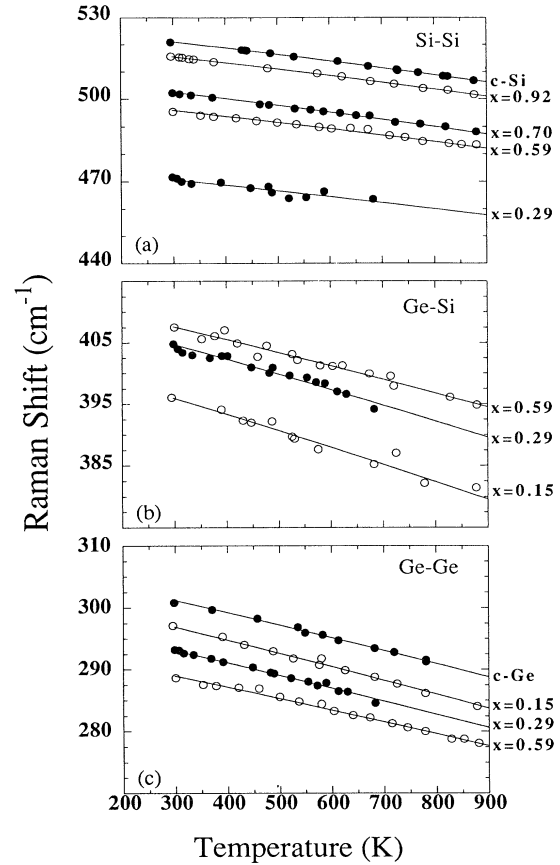
FIG. 3. Raman shifts of the three \text{Ge}_{1-x}\text{Si}_x alloy modes as a function of temperature, for different alloy concentrations. The experimental uncertainty in the shift is \pm 0.25 \text{ cm}^{-1} for T < 600 \text{ K} , and \pm 0.50 \text{ cm}^{-1} for T > 600 \text{ K} . The solid lines are fits using Eqs. (1)–(4) with parameters given in Table II for each mode and composition.
